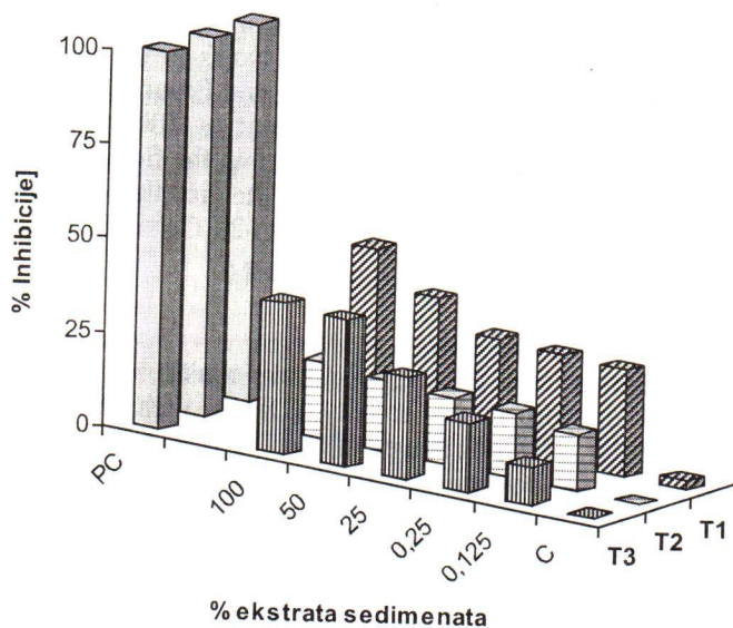
Fig. 2. Inhibition of microbial dehydrogenase synthesis according to the concentration of extracts sediments (DHA test) applied in Arthrobacter globiformis microbial culture. Three investigated sites were compared: T 1 Raduš, T 2 Middle lake, T 3 Mouth River Moraca (C- controle; PC- positive controle)
