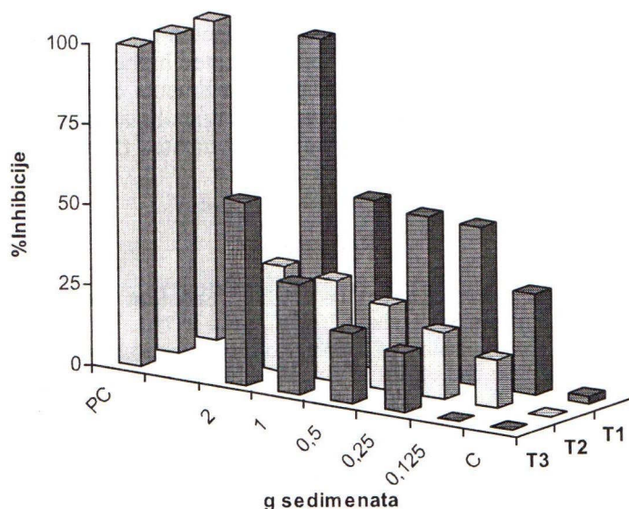
Fig. 3. Inhibition of microbial dehydrogenase synthesis according to the concentration of sediment solid phase (DHA contact test) applied in Arthrobacter globiformis microbial culture. Three investigated sites were compared: T 1 Raduš, T 2 Middle lake, T 3 Mouth River Moraca (C- controle; PC- positive controle)
