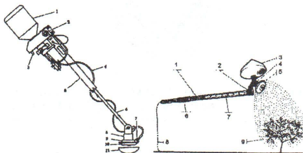
Drawing 2. Manual battery sprayer ULV with rotation nozzle producing 250 \mu\text{m}
