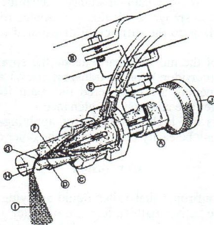
Drawing 6 Airtec sprayer
