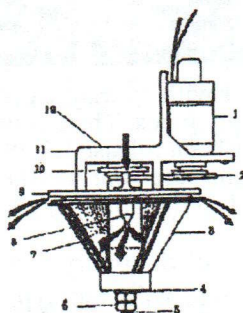
Drawing 4. The Scheme illustrating manifold sprayer work mode 1-12 V motor; 2-three-level drive belt; 3-external conus (disc); 4-Bottom bearing; 5-Central axle; 6-Blockage nut; 7-Internal conus; 8-Feed jet unit; 9-Upper plate; 10-Three-speed belt disc : 11-Main support 12-upper bearing
