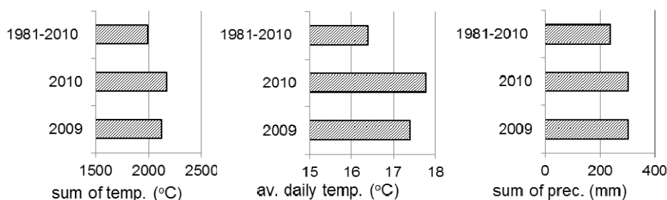
Figure 1. Meteorological data for onion growing seasons (2009, 2010, long-term average, Smederevska Palanka, 20 March – 20 July)
